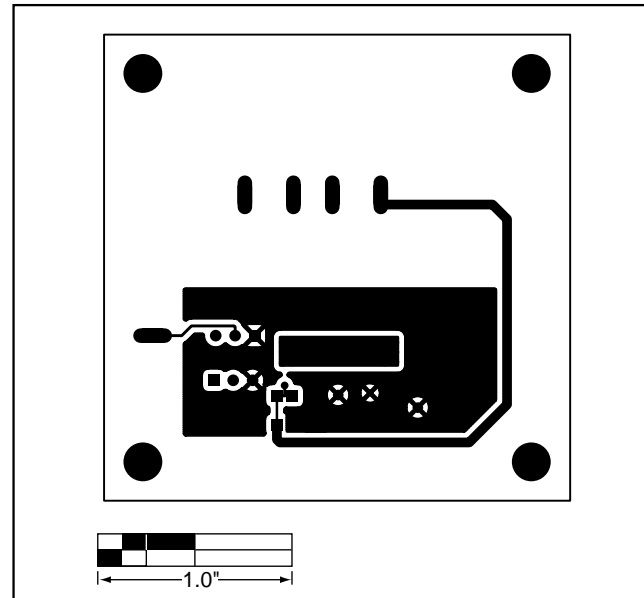
Figure 5. MAX1623 EV Kit PC Board Layout—Solder Side
