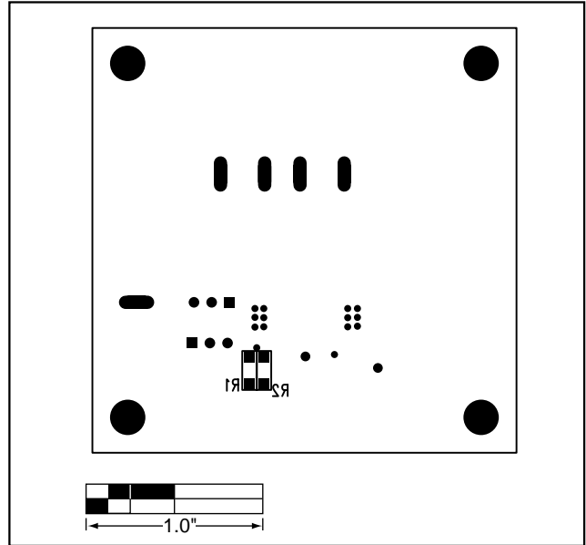
Figure 3. MAX1623 EV Kit Component Placement Guide—Solder Side
